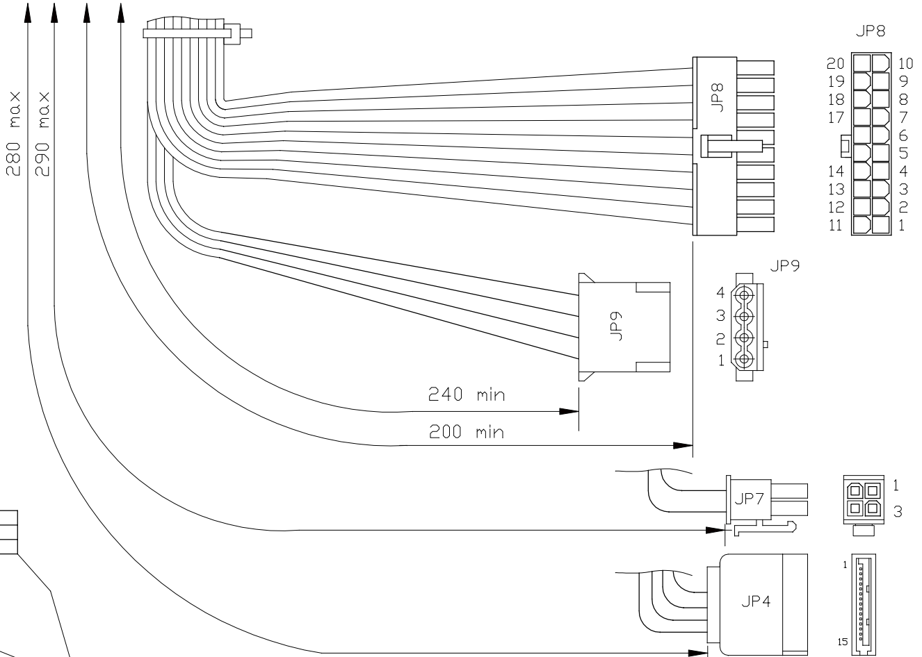
JP9 HDD OUT TH-4F (MOLEX 8981-04P)
